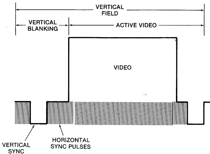
Fig. 8-3. Video waveform for one vertical field.
